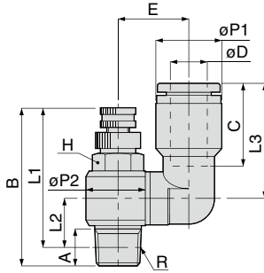
Unified thread type
