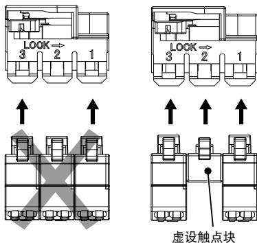
虚设触点块
