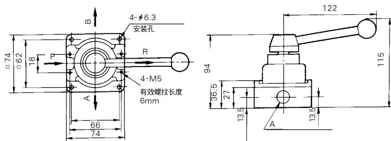
DH300-03/四边接管
