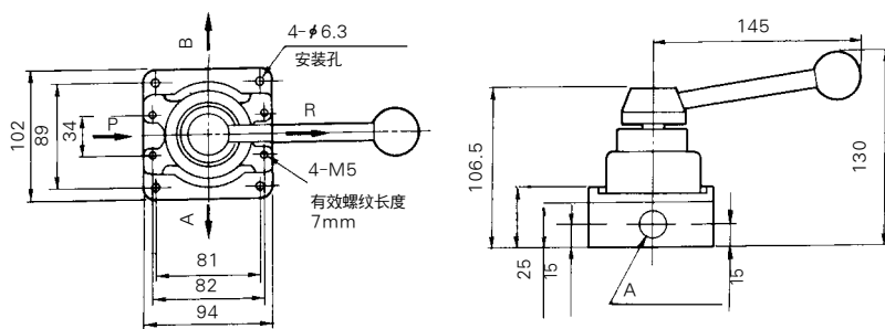
DH400-04/四边接管
