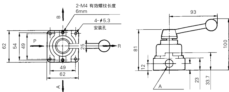
DH200-02/四边接管
